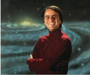
Fig.5 Carl Sagan
